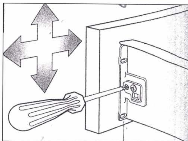
Sidejustering
