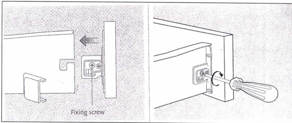
Monter front.
