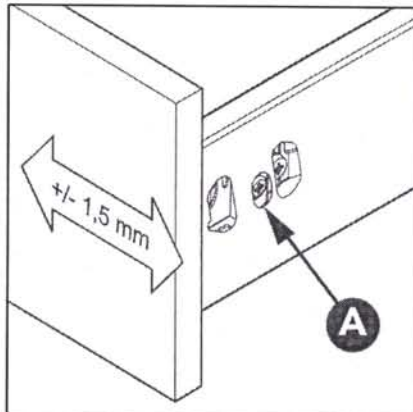
Sidejustering
